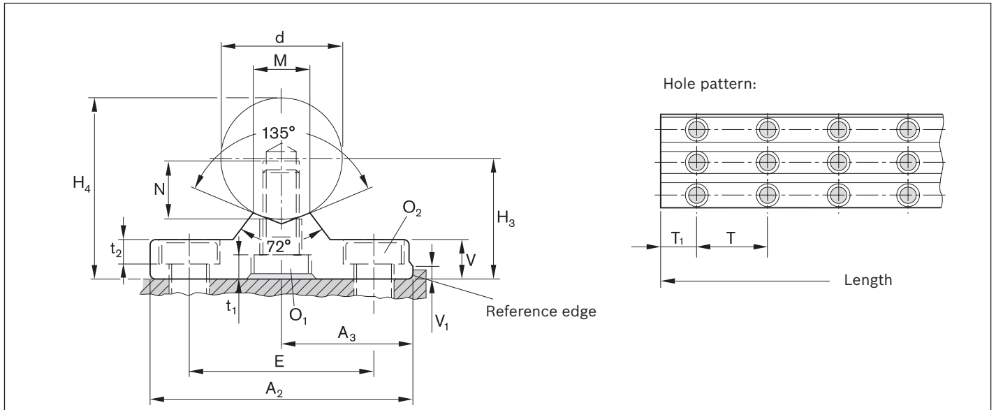
Dimensions (mm)
