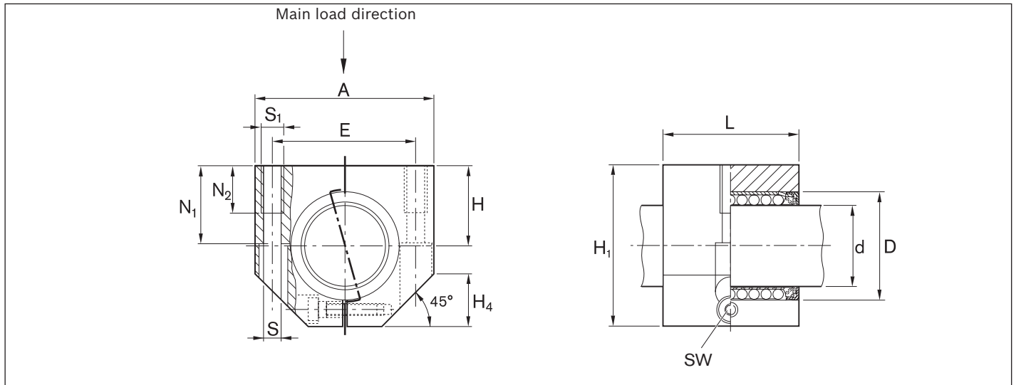
Dimensions (mm)
