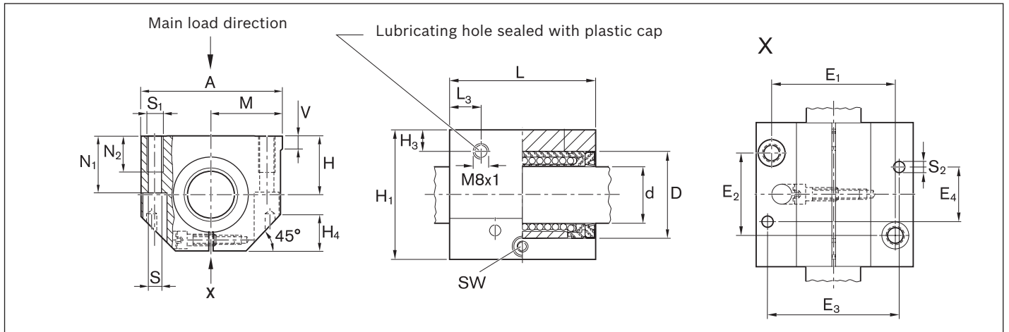
Dimensions (mm)
