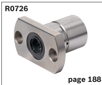
Torque-resistant linear bushing Miniature flanged, with four ball guide grooves
