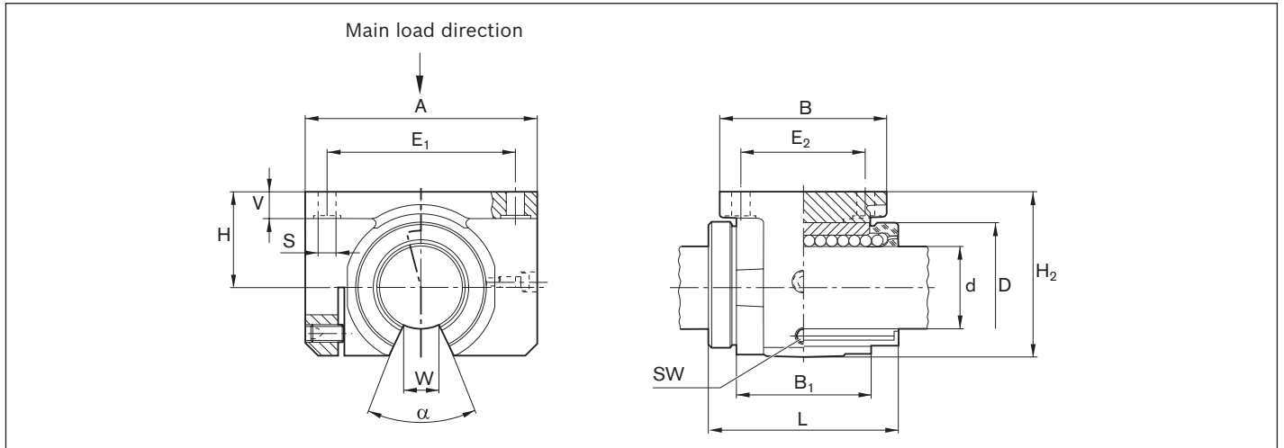
Dimensions (mm)
