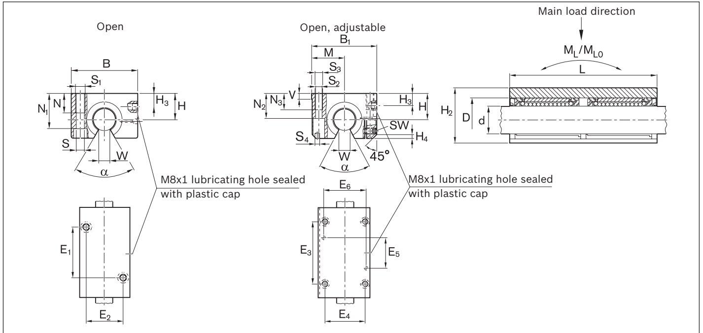
Dimensions (mm)
