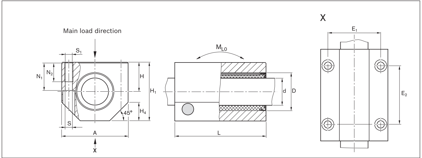
Dimensions (mm)
