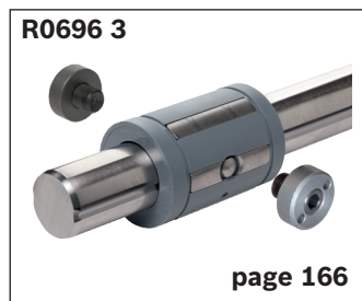
Torque-resistant linear bushing type 2, two ball guide grooves
