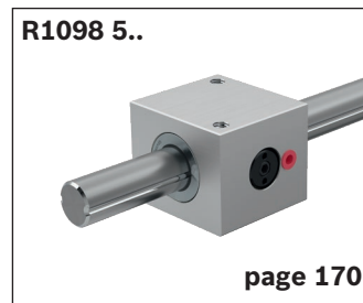
Type 2: Two ball guide grooves
