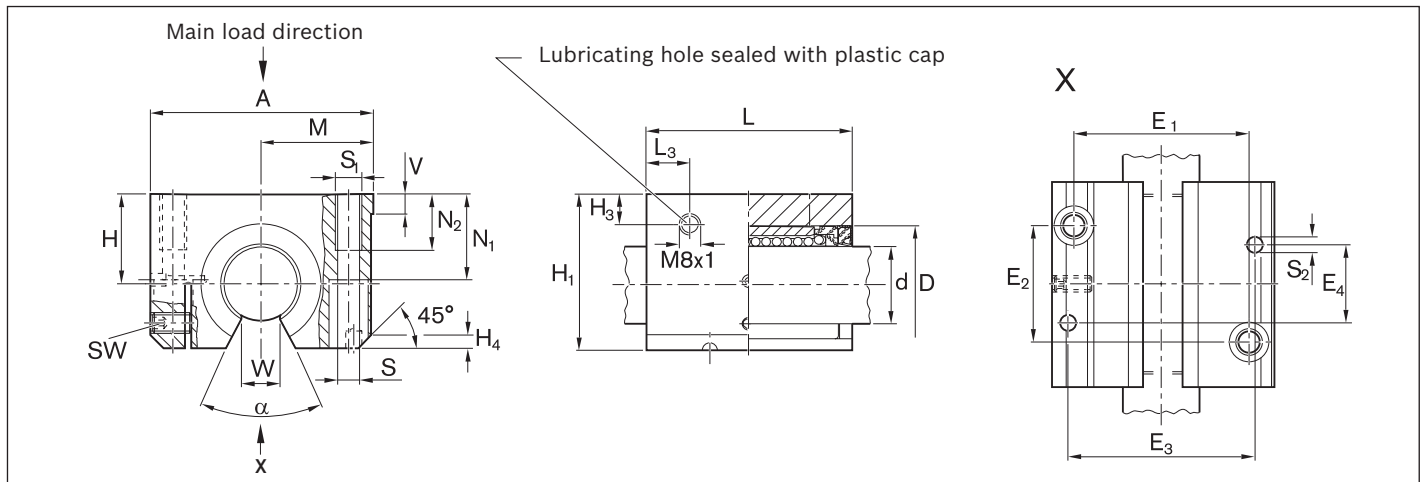
Dimensions (mm)
