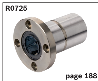
Torque-resistant linear bushing Flanged, with four ball guide grooves
