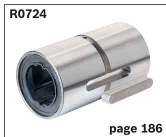
Torque-resistant linear bushing Four ball guide grooves
