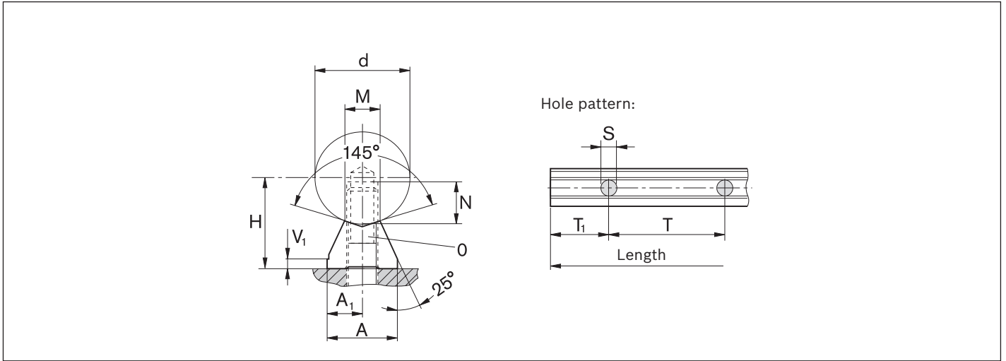
Dimensions (mm)
